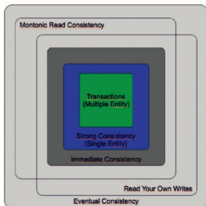
Abb. 4: Eventual Consistency
